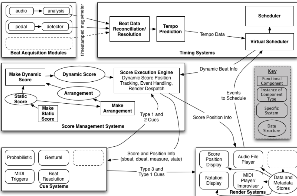
Figure 1: A Reference Architecture for HCMP
