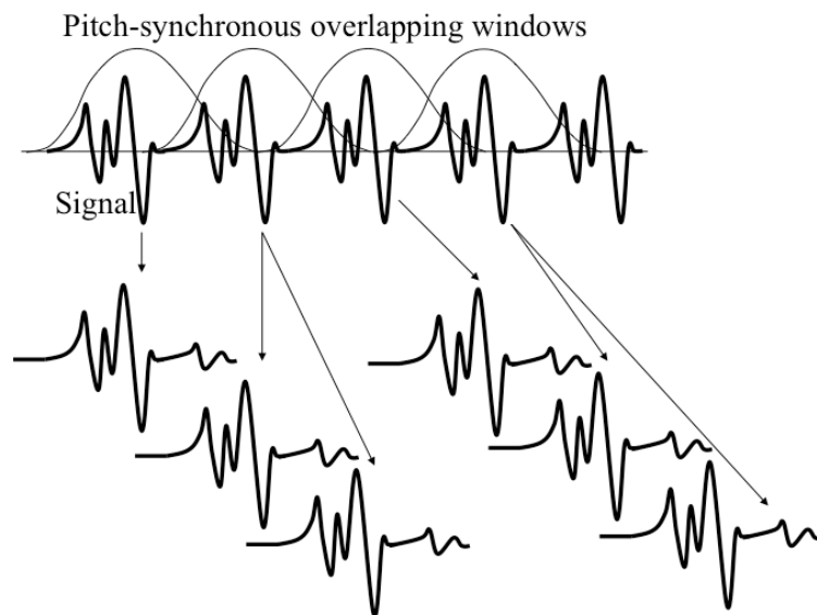
Figure 2. Pitch-Synchronous Overlap Add (PSOLA)
